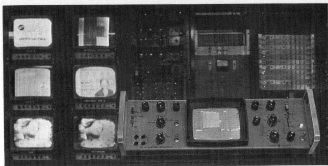
Fig. 2. New TV Waveform Oscilloscope in typical TV control room. Waveform shown is multiburst signal used for checking frequency response of network.
