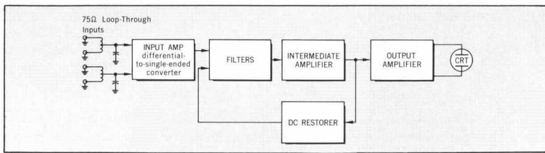
Fig. 4. Block Diagram of Vertical Amplifier in hp - Model 191A Television Waveform Oscilloscope. Passive filters of special design give accurately-shaped responses with high stability. Differential-to-single-ended input amplifier permits use of more stable single-ended filters, has high common mode rejection over wide frequency range.
